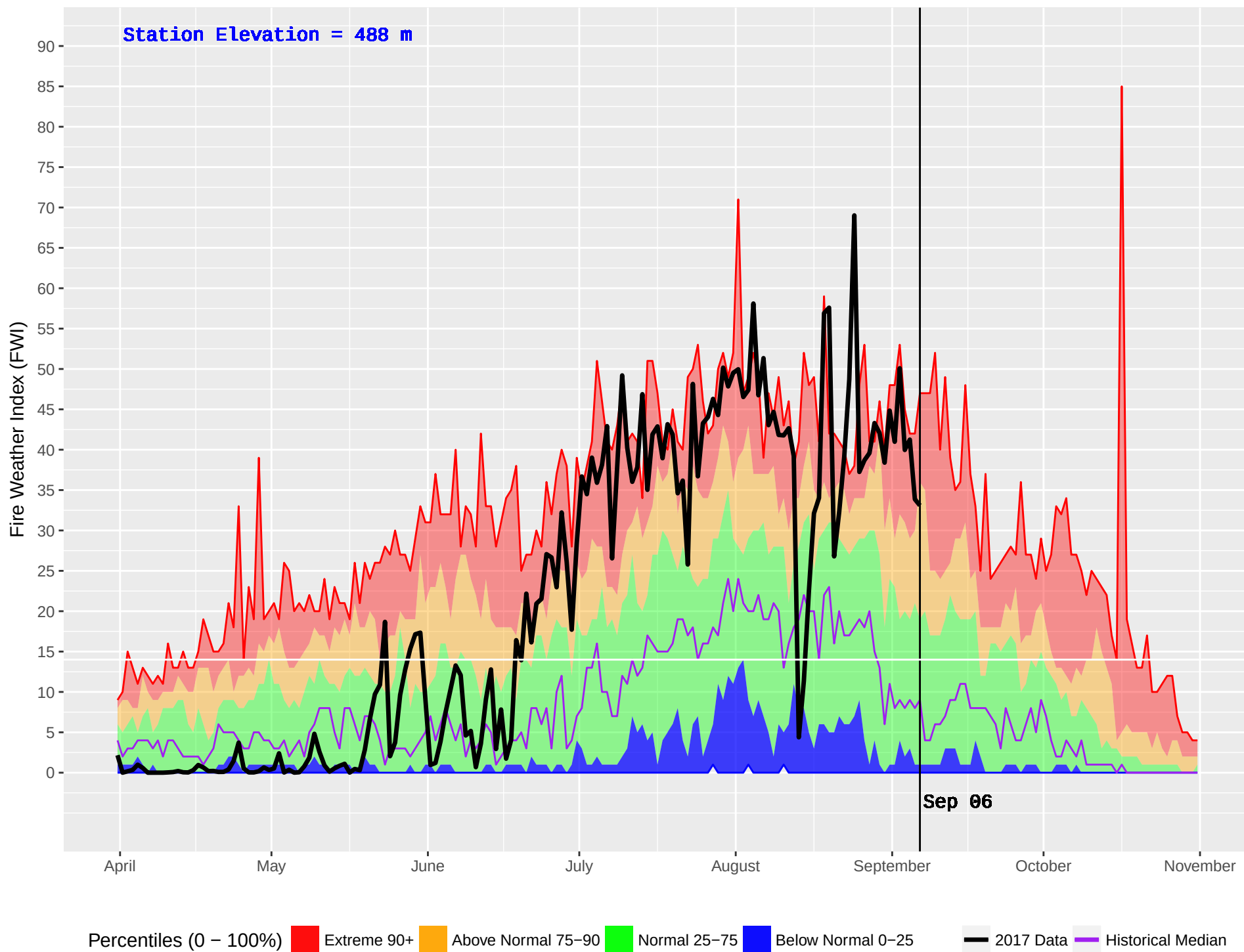
MABEL LAKE 2 (362) : Historical (1987–2016) and Current (2017) Noon Fire Weather Index (FWI)
