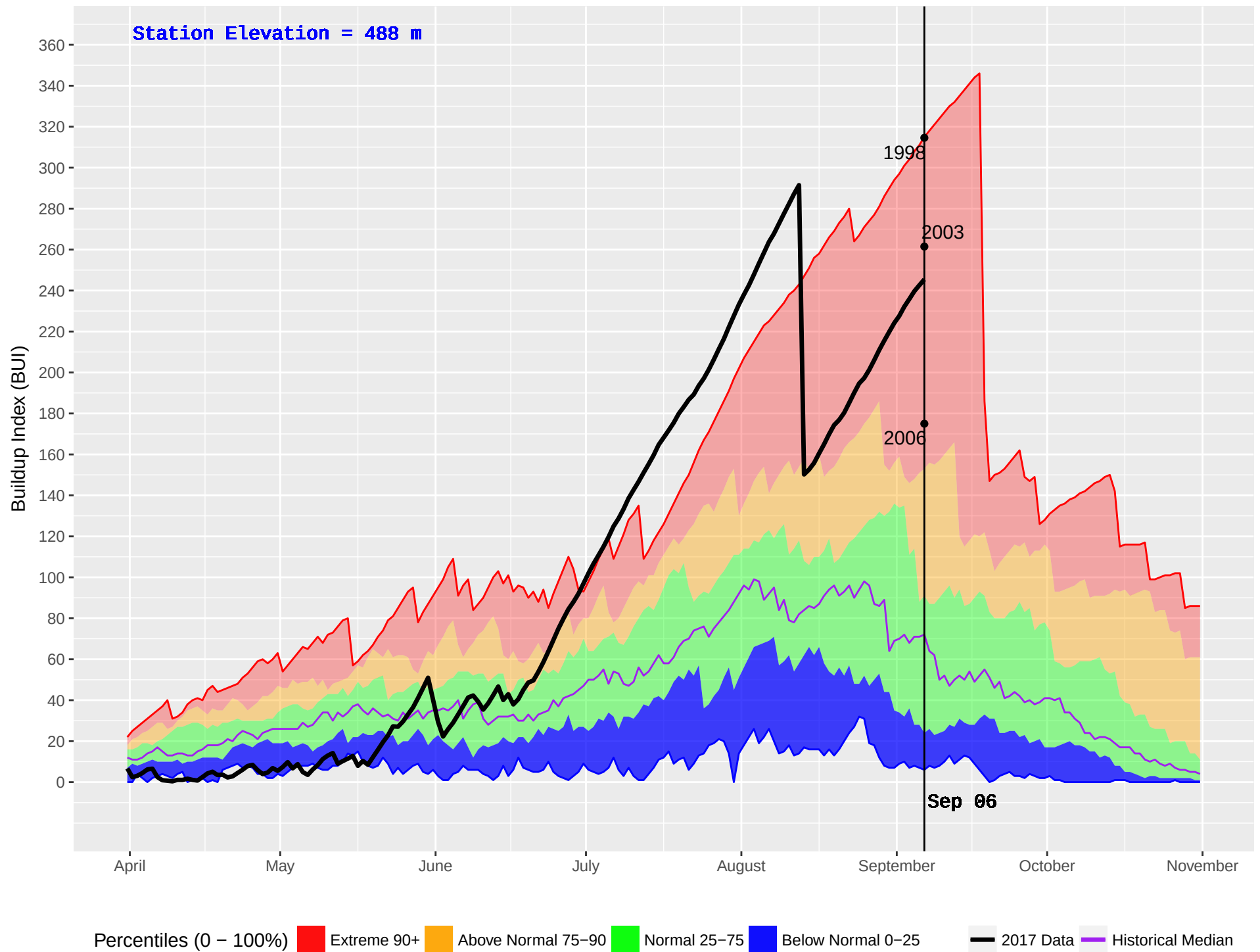
MABEL LAKE 2 (362) : Historical (1987–2016) and Current (2017) Noon Buildup Index (BUI)
