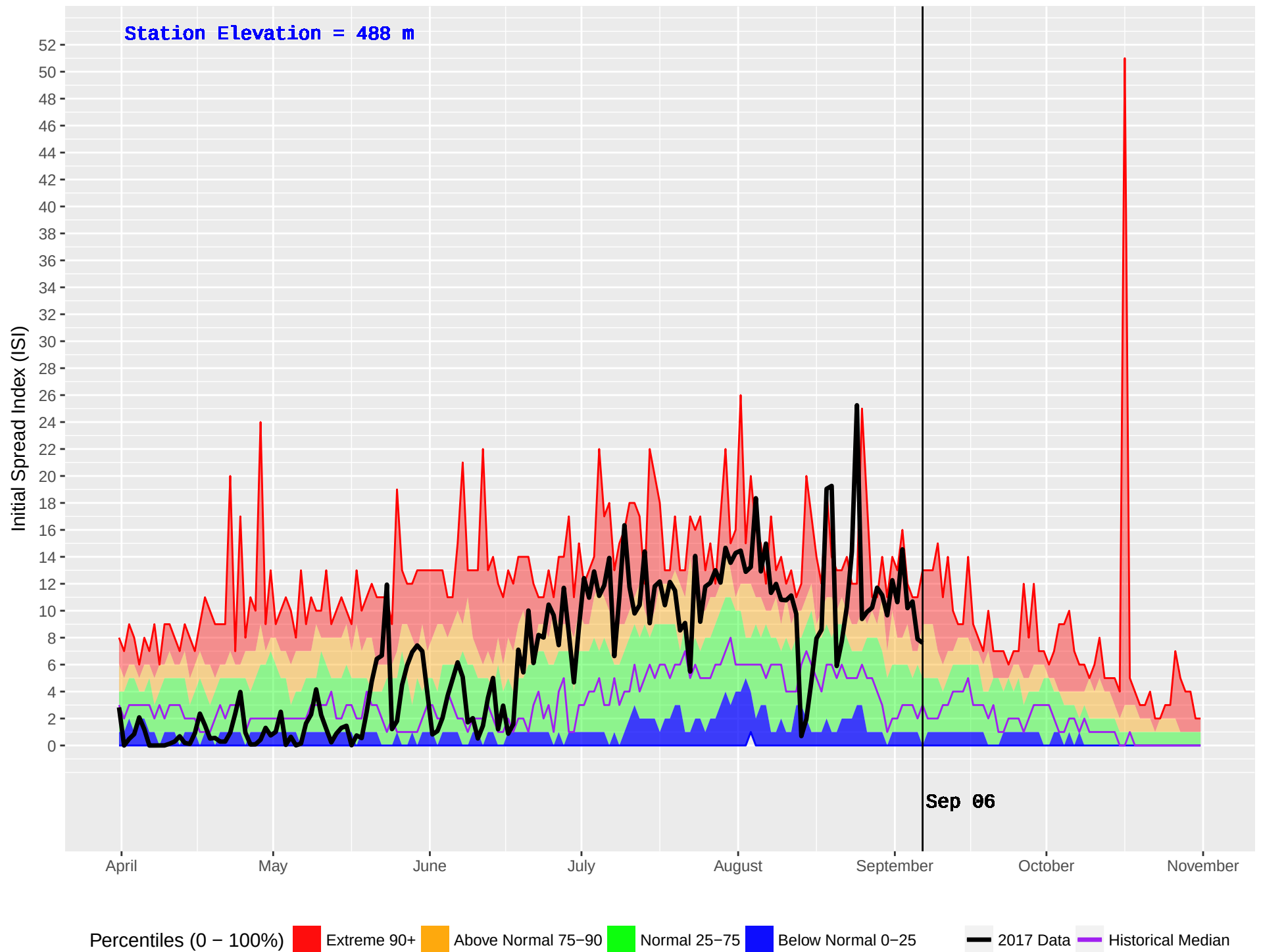
MABEL LAKE 2 (362) : Historical (1987–2016) and Current (2017) Noon Initial Spread Index (ISI)
