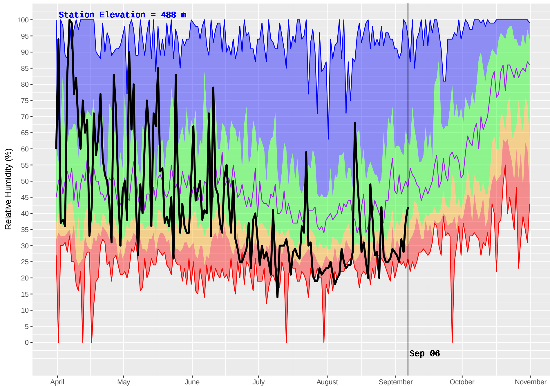
MABEL LAKE 2 (362) : Historical (1987–2016) and Current (2017) Noon Relative Humidity
